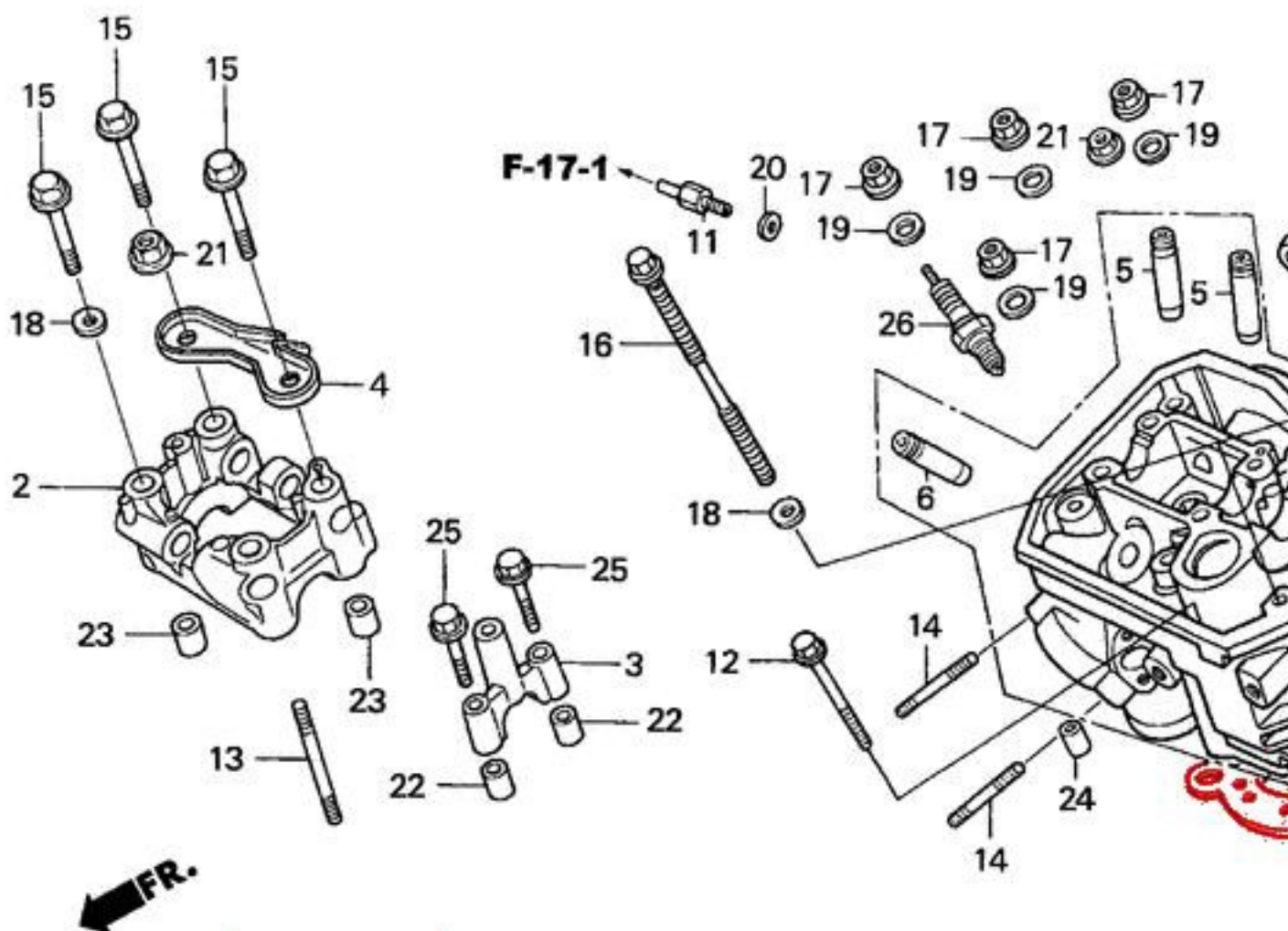
Schemat Honda XL650V
